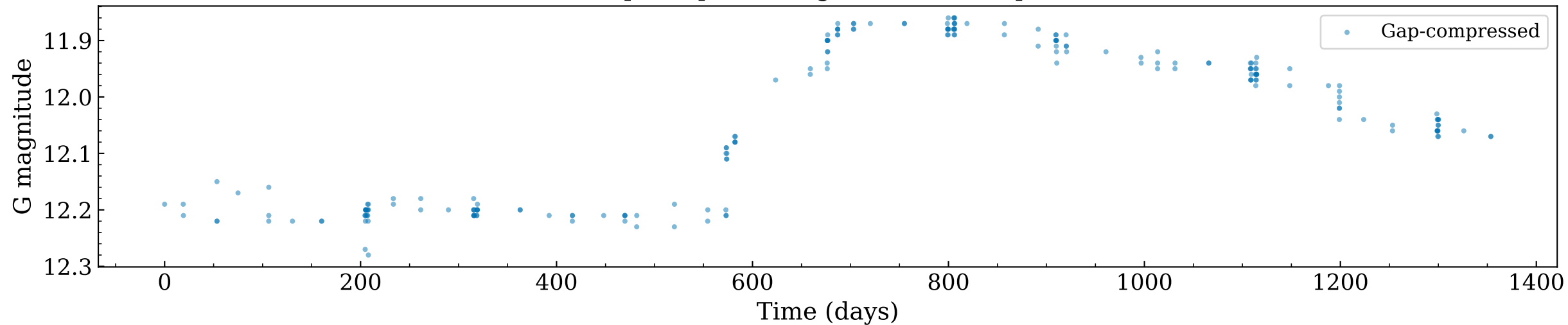
Gap-compressed light curve (GP input)
