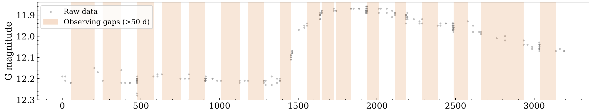
Original Gaia light curve — Gaia19bzu
