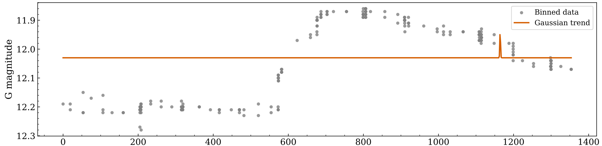
Gaussian trend — Gaia19bzu
