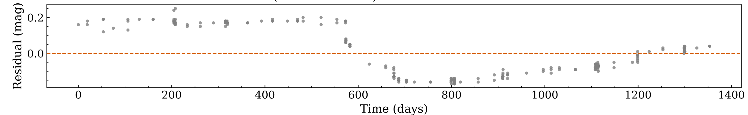
Residual (data – Gaussian) — this is what the GP will model
