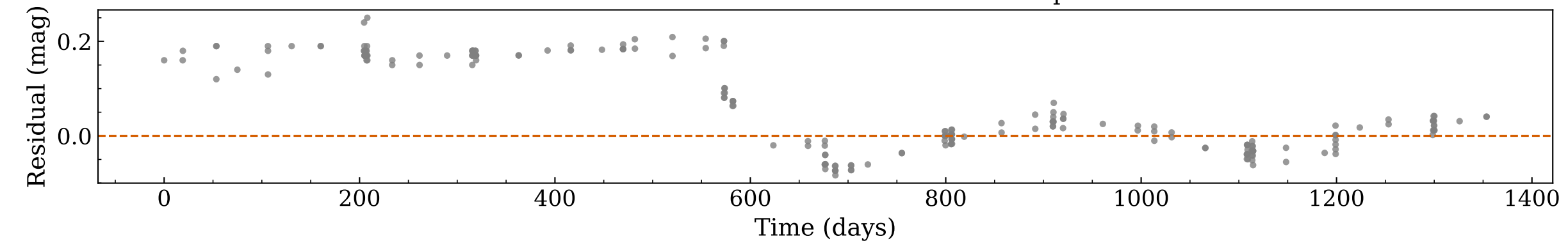
Residual after trend subtraction — GP input
