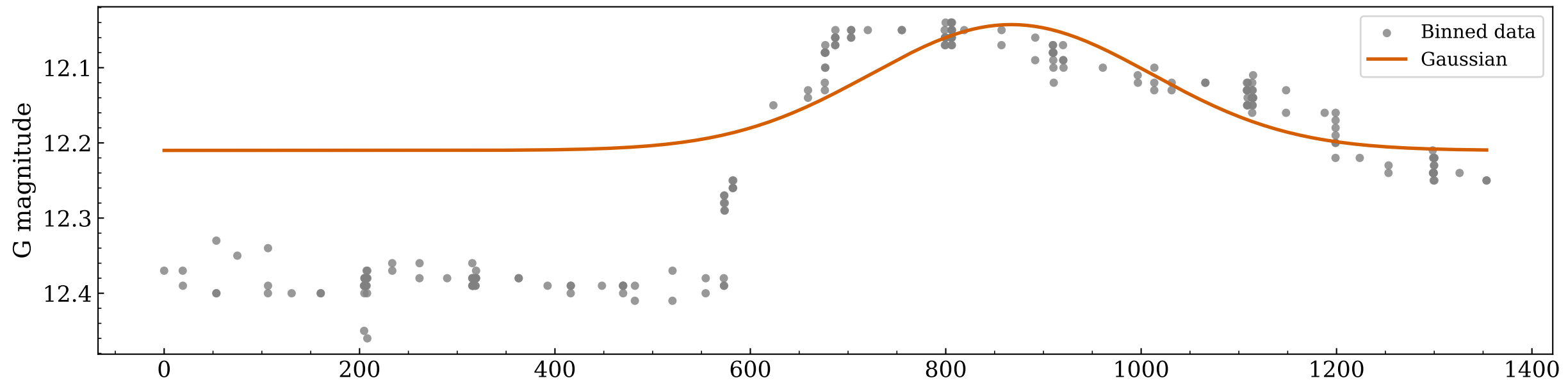
Gaussian trend fit — Gaia19bzu
