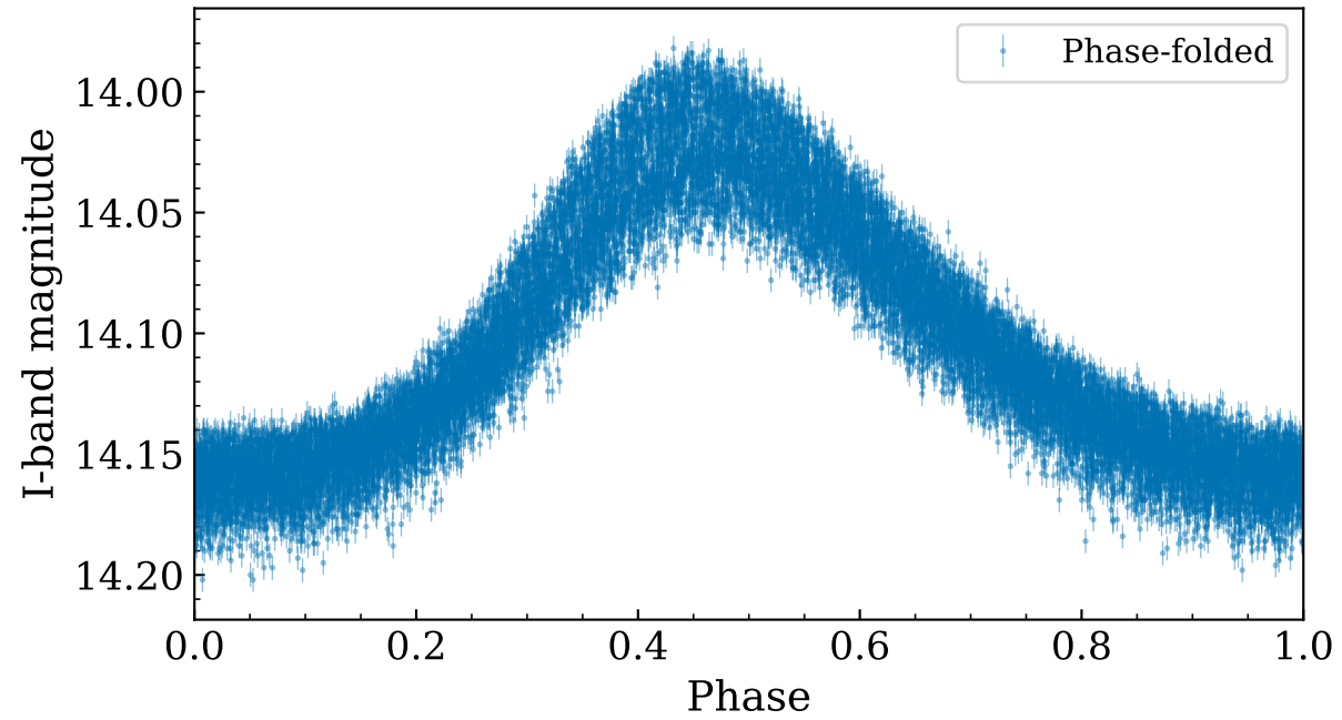
Phase-folded ( P = 0.2865 d)
