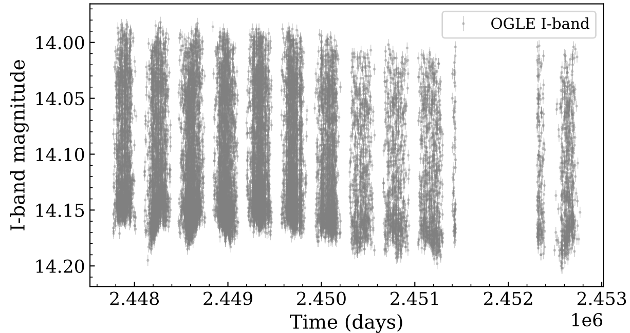
Raw light curve — OGLE-BLG-CEP-019
