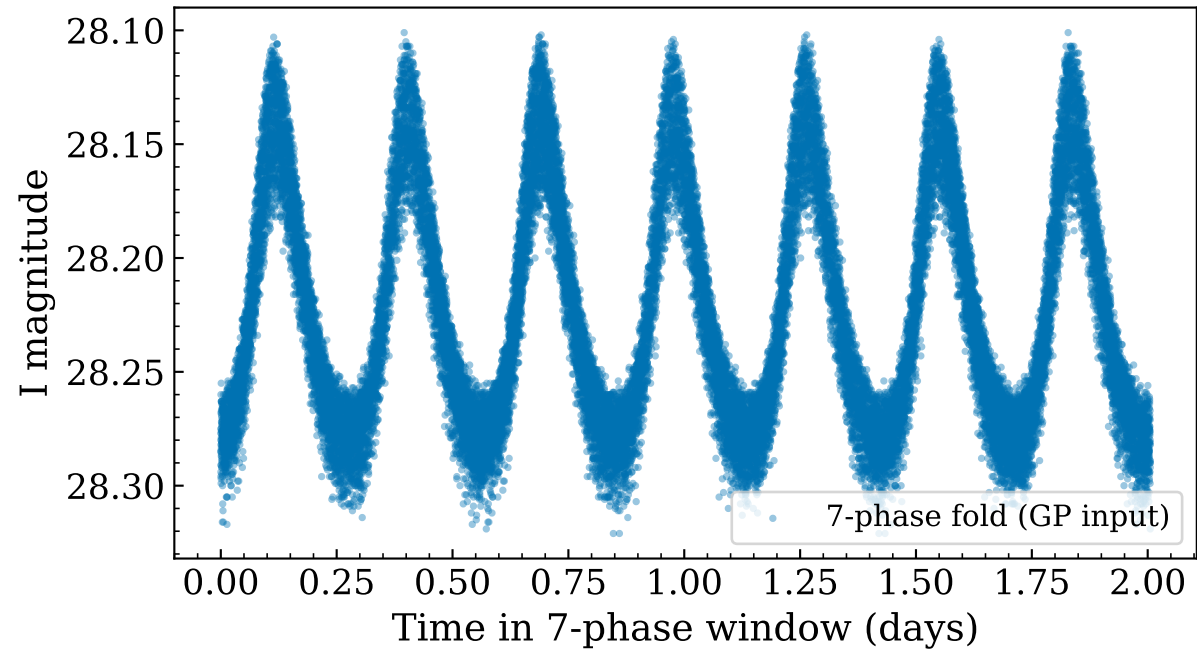
Multi-phase fold ( n = 7 )
