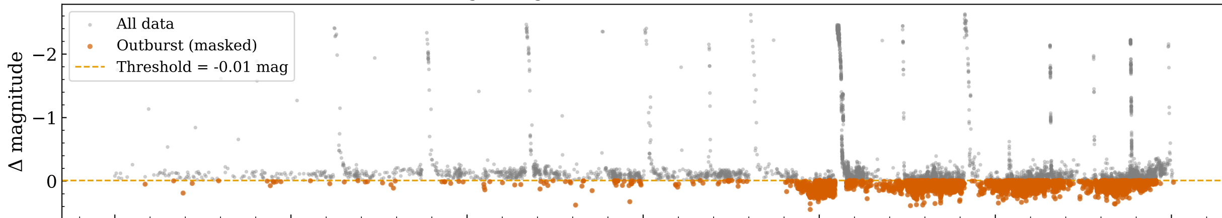
Original light curve — OGLE-BLG-DN-0001
