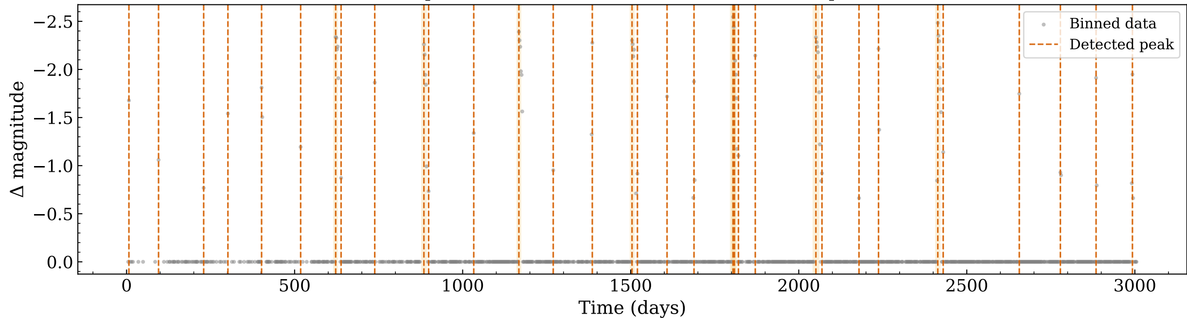
Multi-scale peak detection — OGLE-BLG-DN-0001 (33 peaks found)
