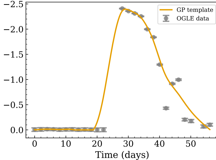
Outburst peak t_0 = 2051.0 d
