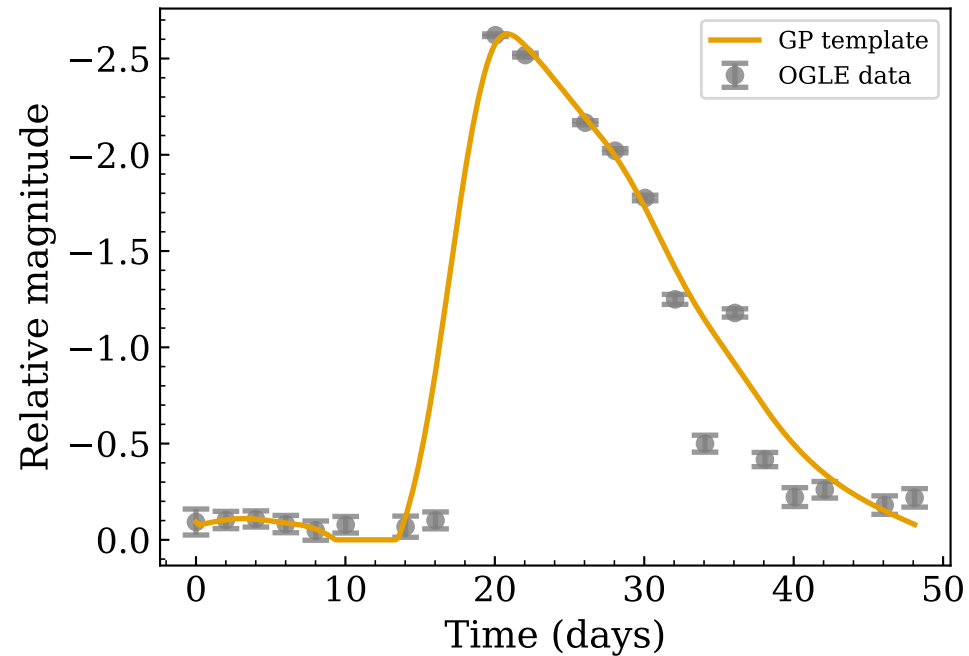
Outburst peak t_0 = 1808.5 d
