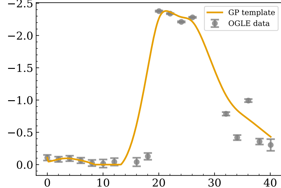
Outburst peak t_0 = 1504.0 d
