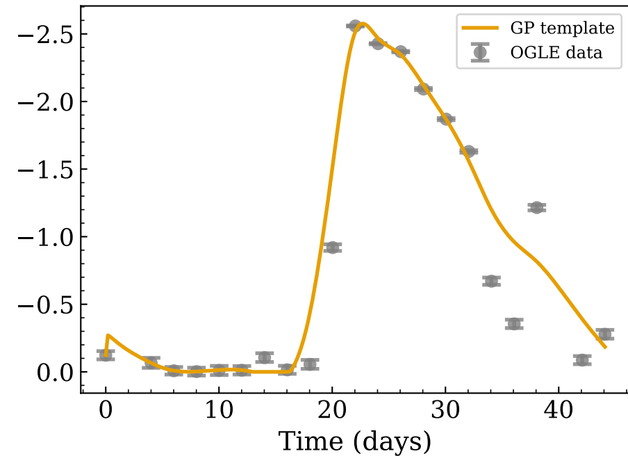
Outburst peak t_0 = 2413.7 d
