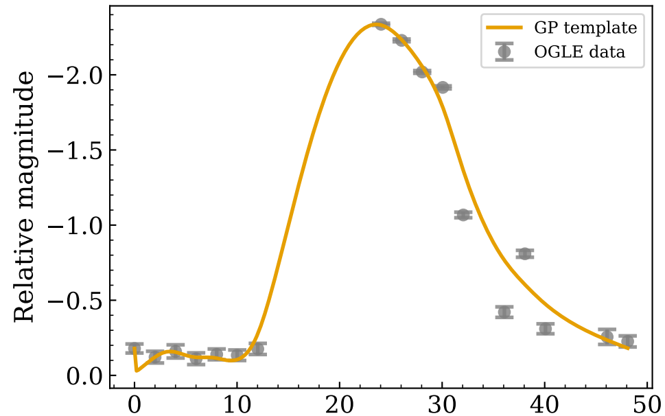
Outburst peak t_0 = 884.7 d
