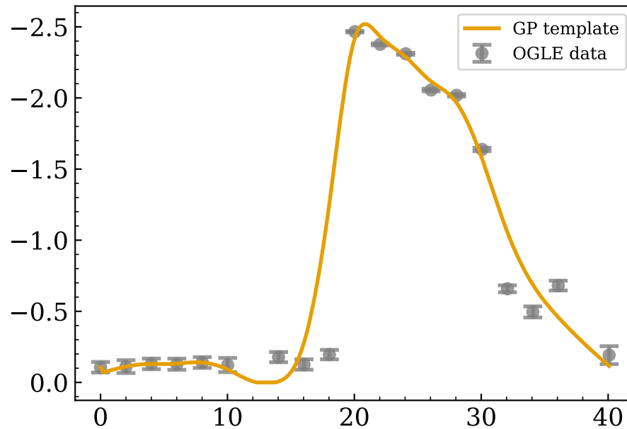
Outburst peak t_0 = 1167.3 d
