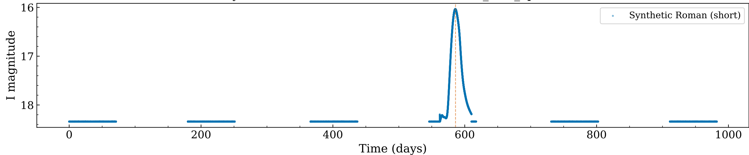
Synthetic Roman LC — OGLE-BLG-DN-0001_ind0_1peaks
