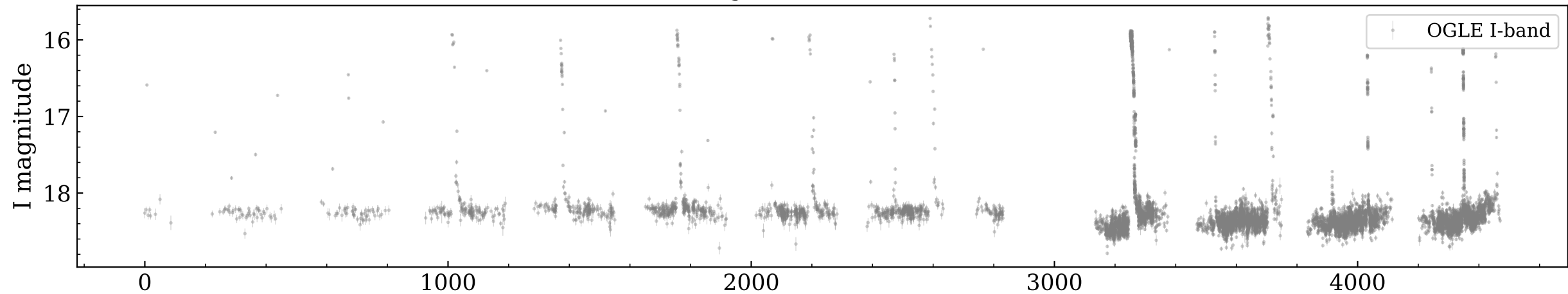
Observed OGLE light curve — OGLE-BLG-DN-0001
