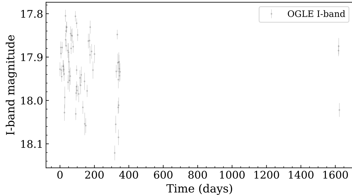
Raw light curve — OGLE-BLG-ECL-100098
