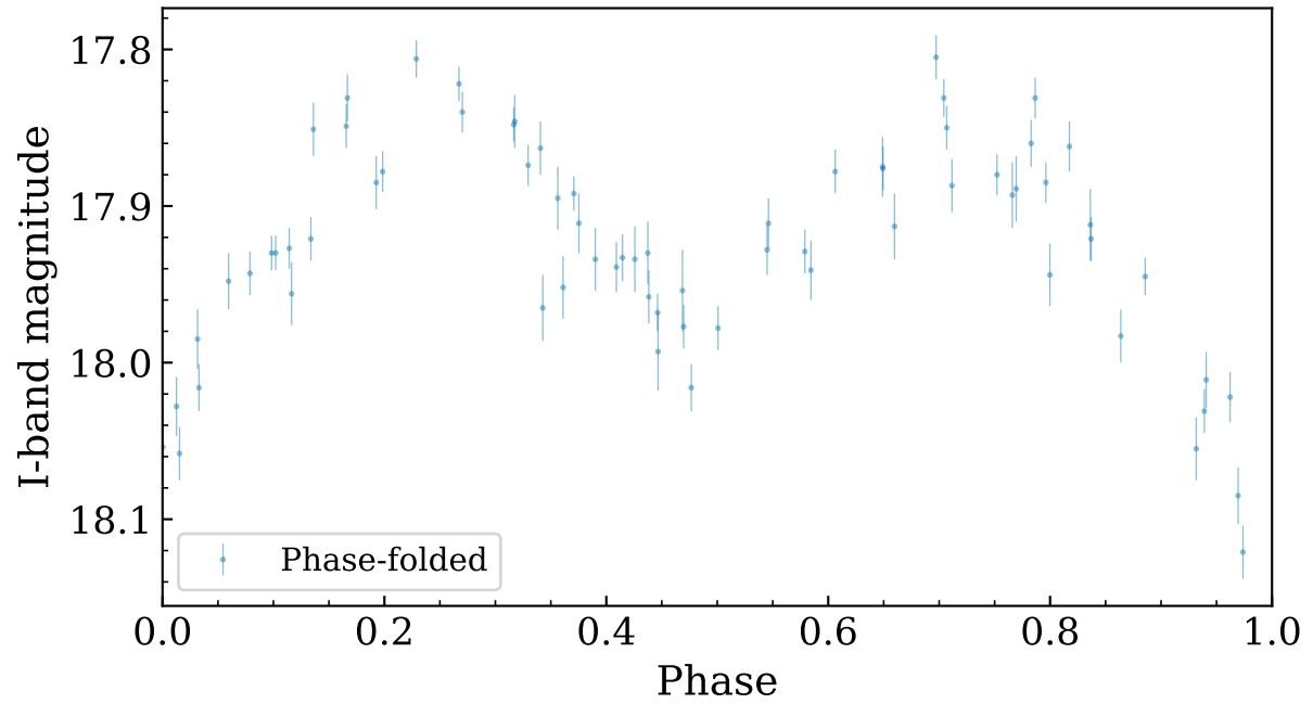
Phase-folded ( P = 0.5479 d)
