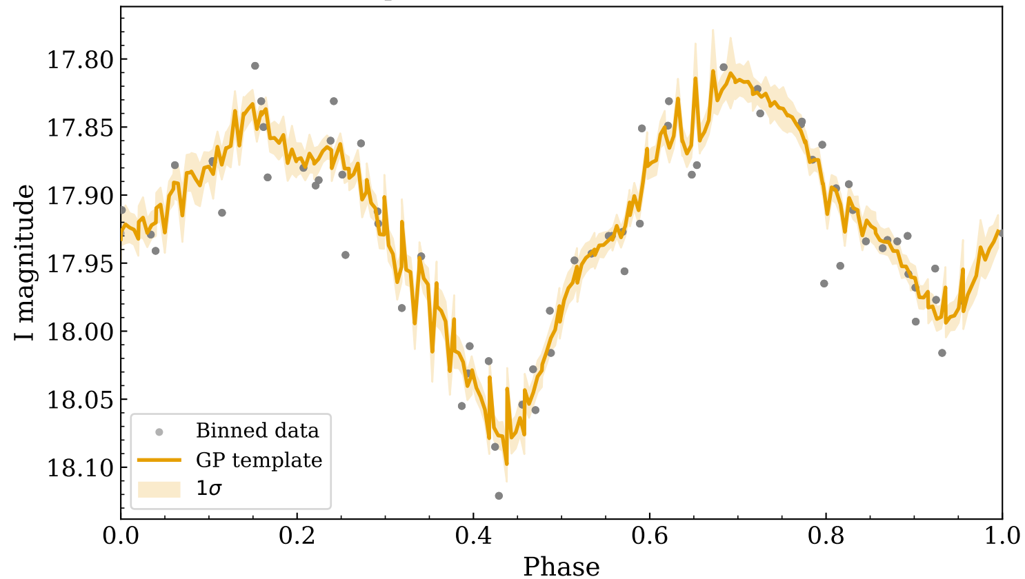
Phase-folded GP template — OGLE-BLG-ECL-100098 ( P = 0.5479 d)
