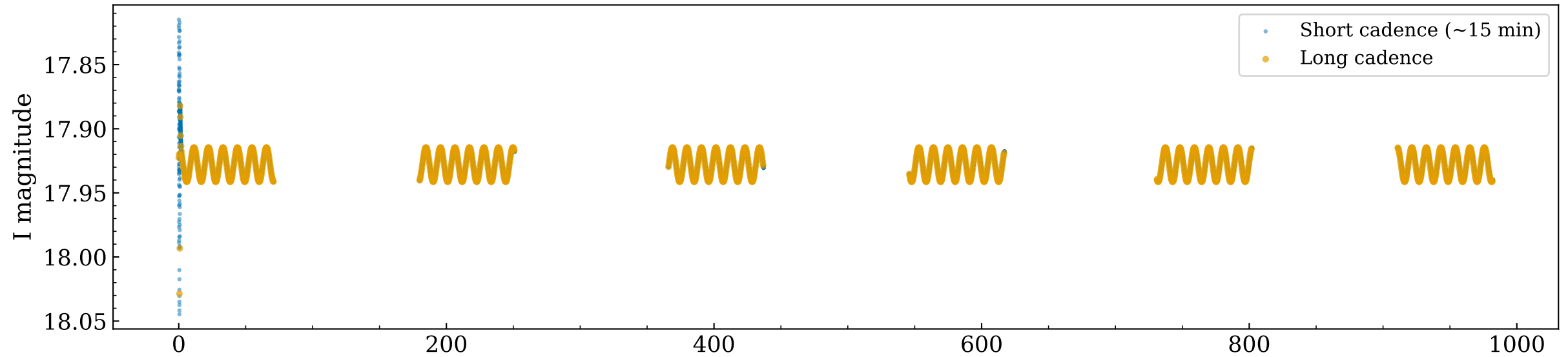
Synthetic Roman light curve (time domain) — OGLE-BLG-ECL-100098
