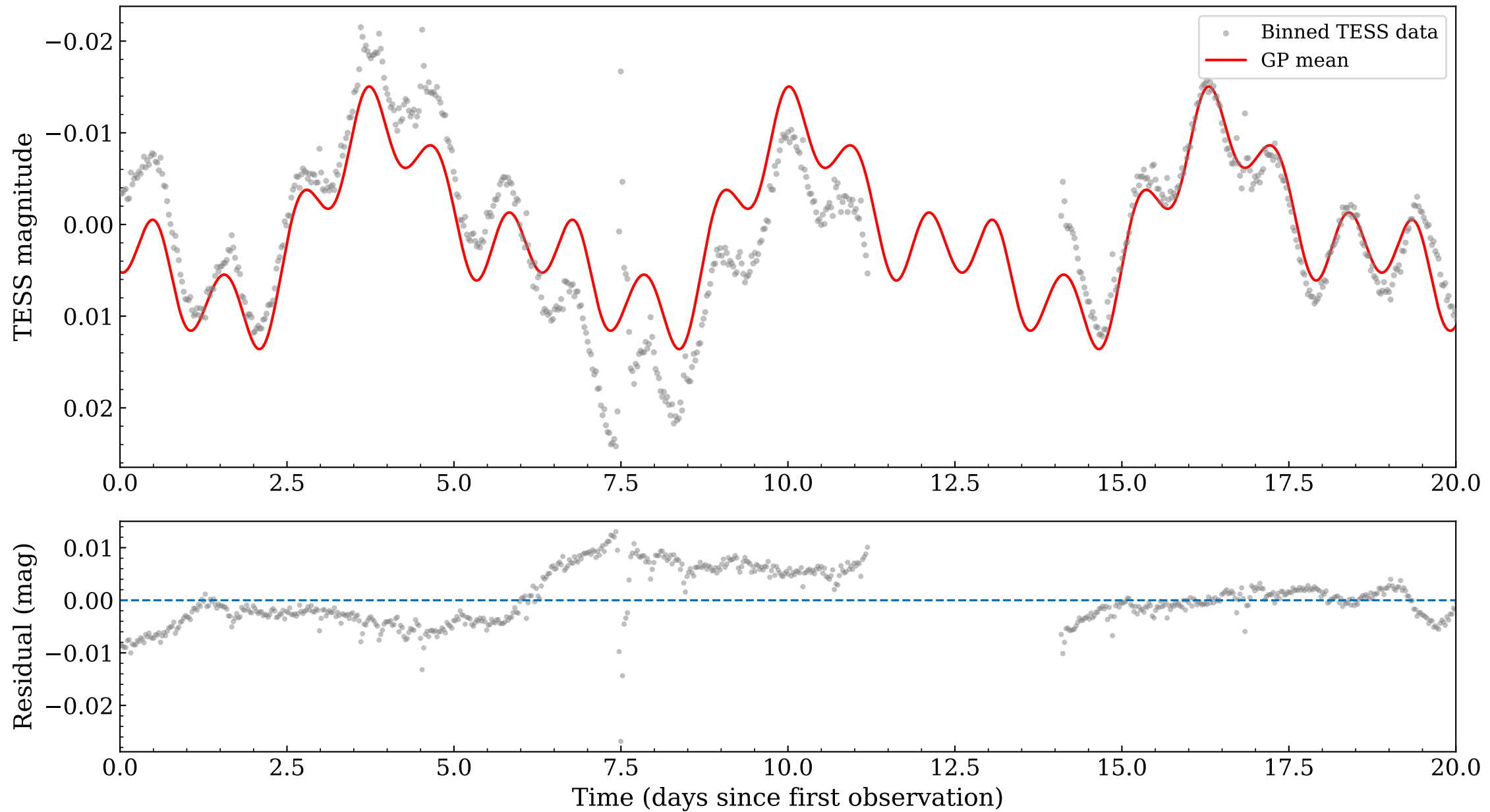
GP baseline fit — TIC 117874959
