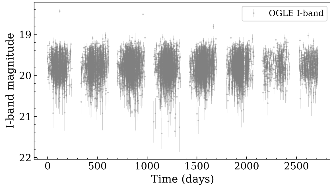
Raw light curve — OGLE-BLG-RRLYR-03350
