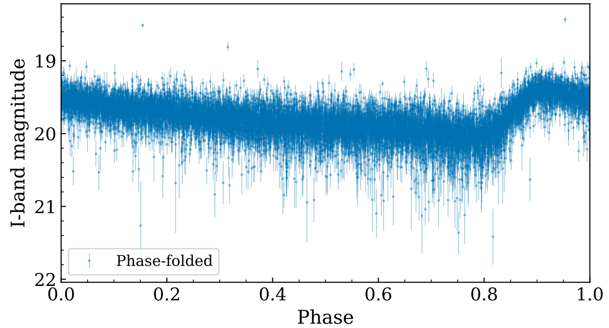
Phase-folded ( P = 0.5148 d)
