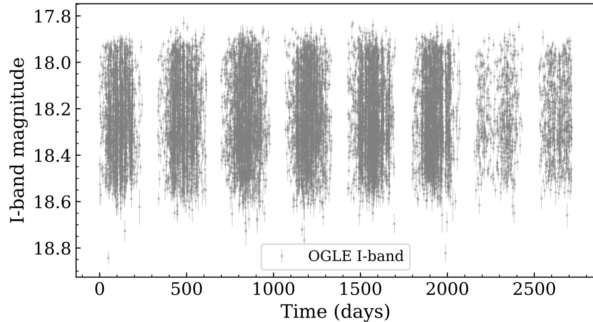
Raw light curve — OGLE-BLG-RRLYR-03609
