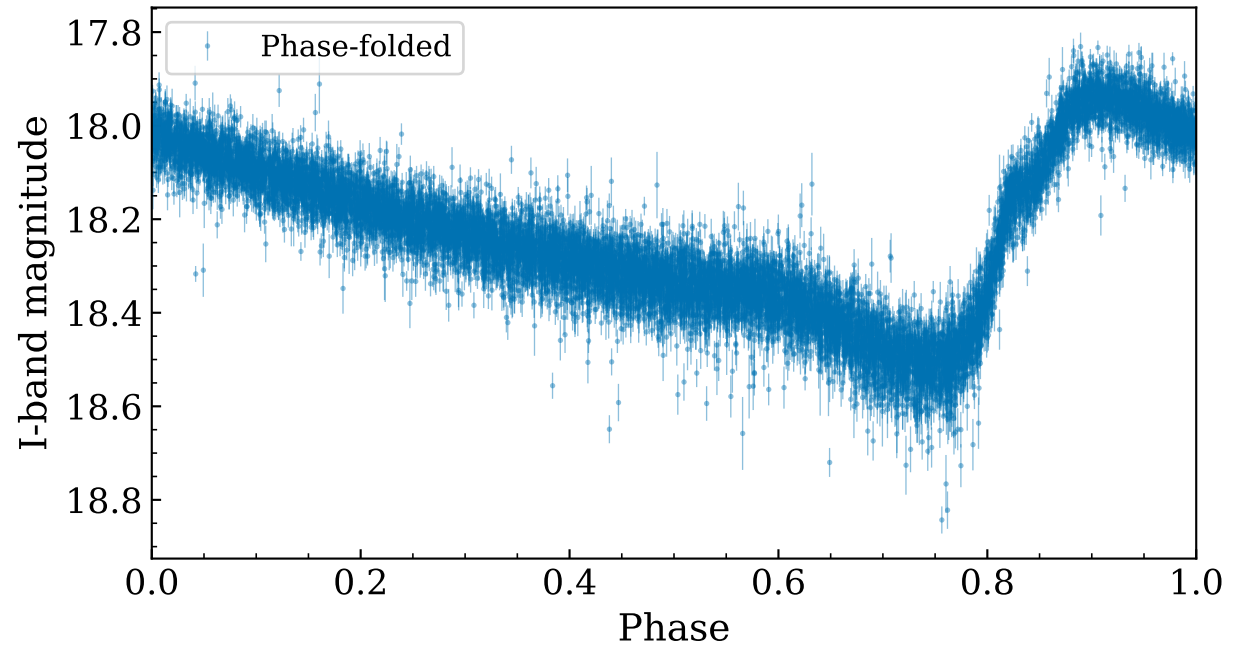
Phase-folded ( P = 0.5579 d)
