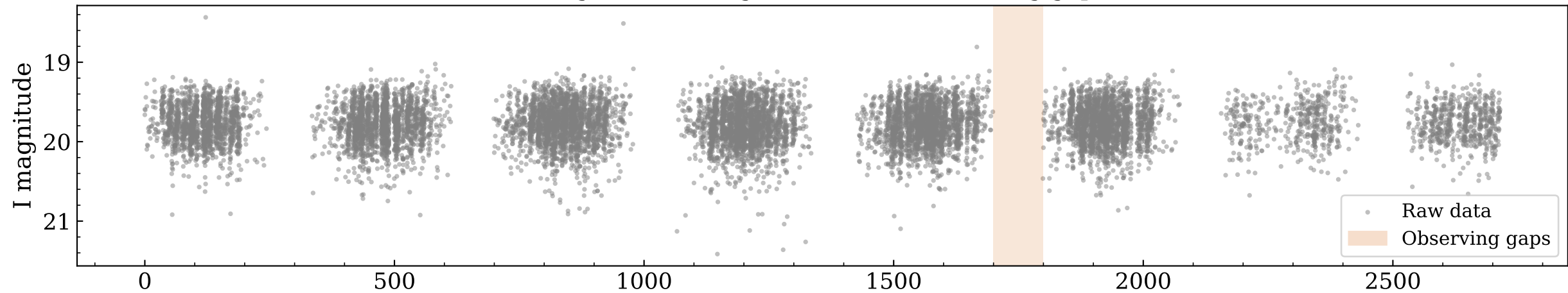
Original OGLE light curve with observing gaps
