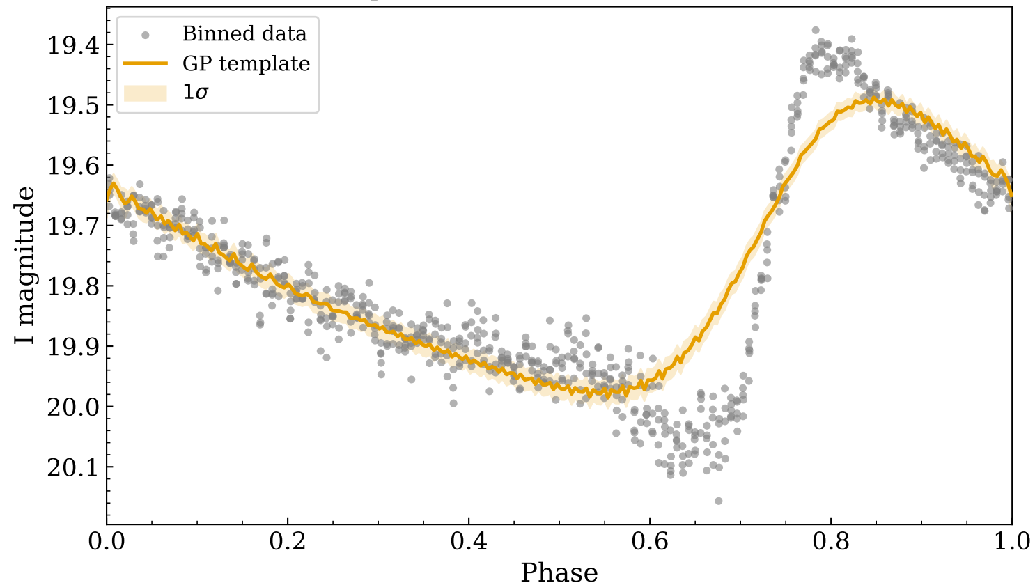
Phase-folded GP template — OGLE-BLG-RRLYR-03350 ( P = 0.5148 d)
