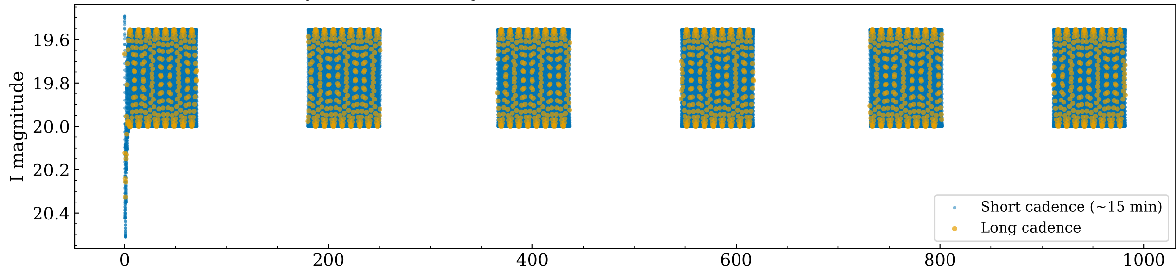
Synthetic Roman light curve (time domain) — OGLE-BLG-RRLYR-03350
