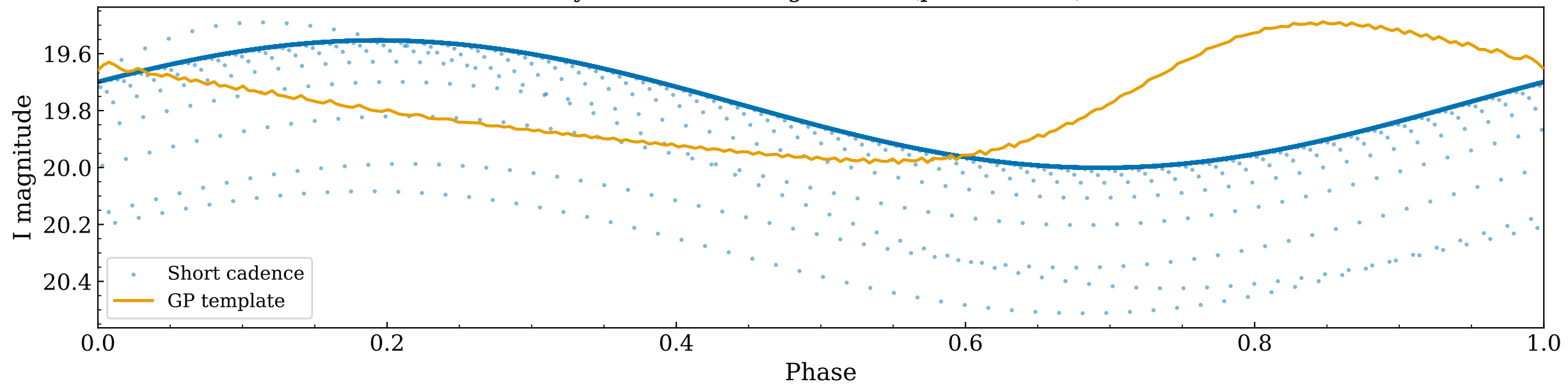
Synthetic Roman light curve (phase-folded)
