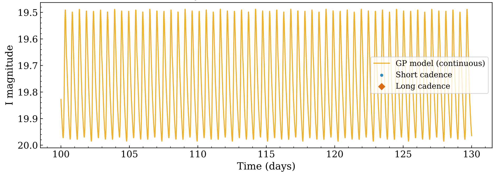
Zoom: 100-130 days — "OGLE-BLG-RRLYR-03350" ( P = 0.515 d)
