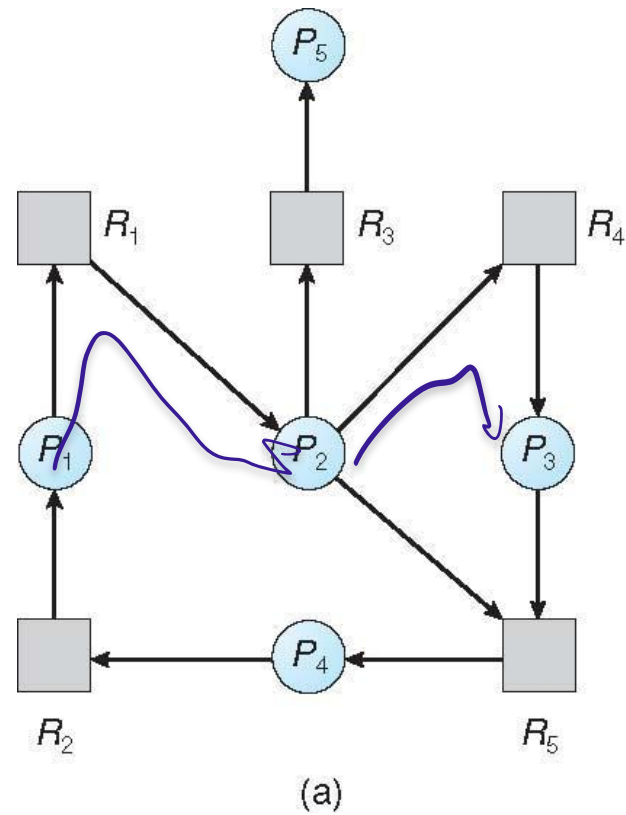
Resource-Allocation Graph
