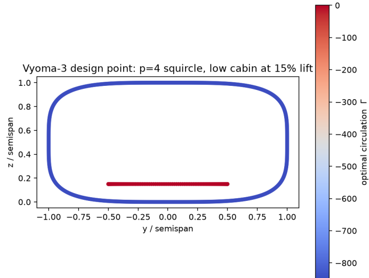
Figure 5: Optimal circulation at the combined design point: p = 4 superellipse, h/b = 0.5 , low-set central body at 15% lift share.
