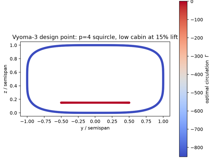
Figure 6: Optimal circulation at the combined design point: p = 4 superellipse, h/b = 0.5 , low-set central body at 15% lift share.
