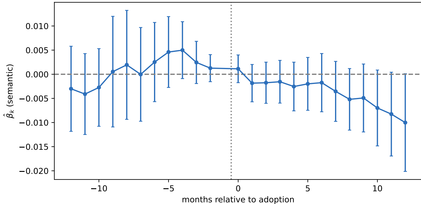
Dynamic DiD event study, enriched panel (k = -12 ... +12)
