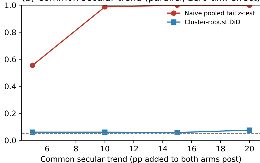
(b) Common secular trend (parallel; zero diff. effect)
