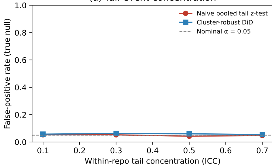
(a) Tail-event concentration
