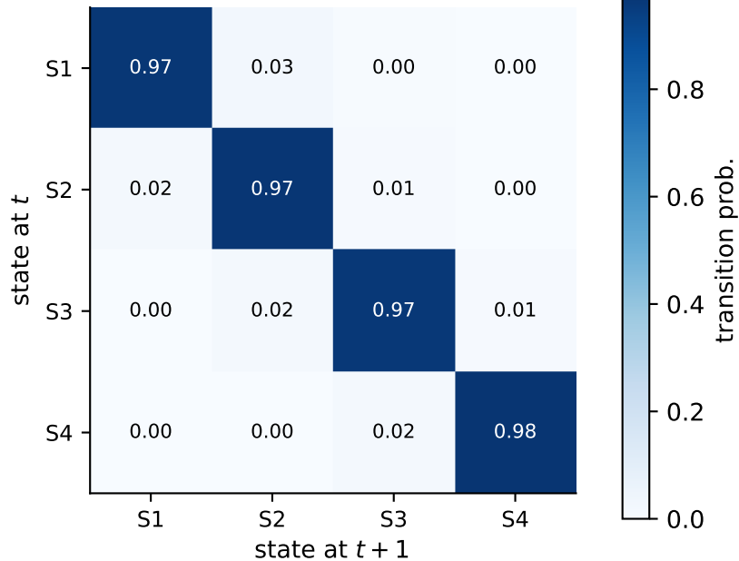
Post-adoption (gap 1 - |\lambda_2| = 0.017 )
