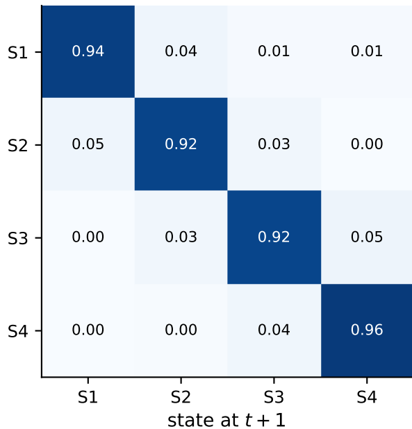
Pre-adoption (gap 1 - |\lambda_2| = 0.036 )
