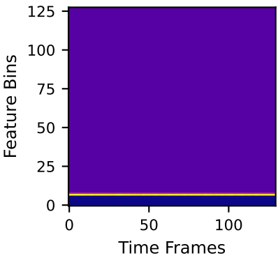
Channel 2: Spectral (128, 130)
