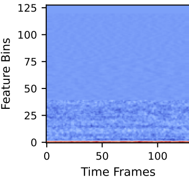
Channel 1: MFCC (128, 130)
