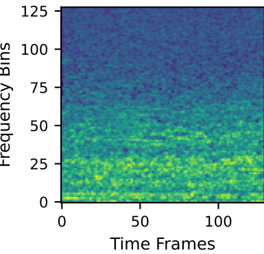
Channel 0: Mel (128, 130)
