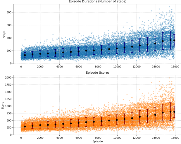
Figure 1: Training metrics of the DQN learning agent. The first plot shows the average steps taken per episode, the second plot shows the average score per episode. Each plots also includes mean and standard deviation computed over last runs.
