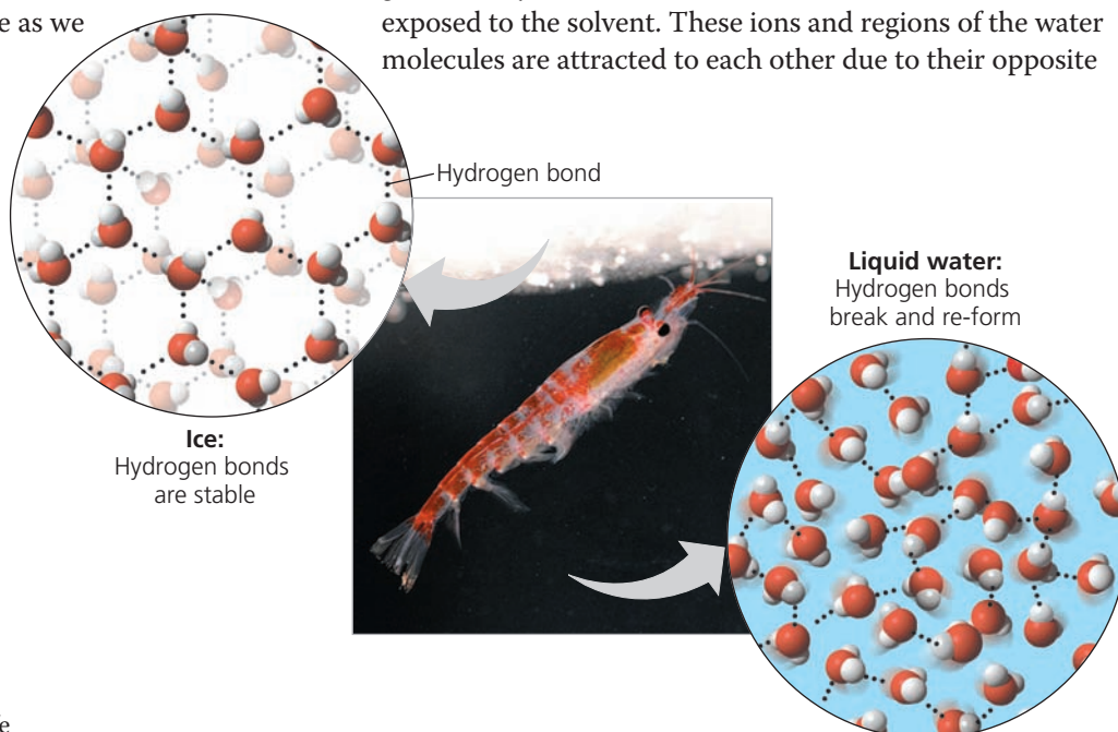
► Figure 3.6 Ice: crystalline structure and floating barrier. In ice, each molecule is hydrogen-bonded to four neighbors in a three-dimensional crystal. Because the crystal is spacious, ice has fewer molecules than an equal volume of liquid water. In other words, ice is less dense than liquid water. Floating ice becomes a barrier that insulates the liquid water below from the colder air. The marine organism shown here is a type of shrimp called krill; it was photographed beneath floating ice in the Southern Ocean near Antarctica.
