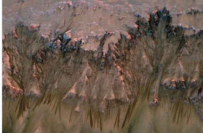
▲ Figure 3.9 Evidence for subsurface liquid water on Mars.
