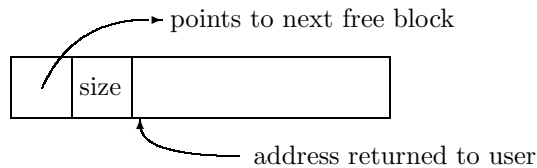
A block returned by malloc
