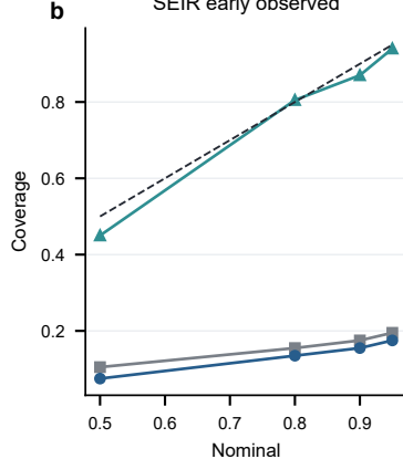
SEIR early observed
