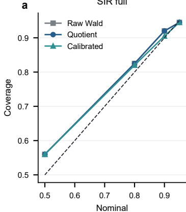
SIR full
