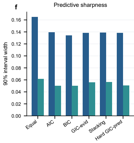
Predictive sharpness
