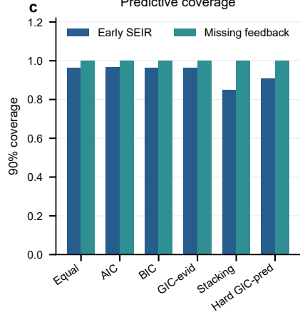
Predictive coverage
