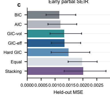
Early partial SEIR
