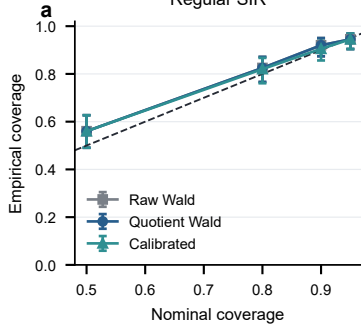
Regular SIR
