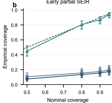
Early partial SEIR
