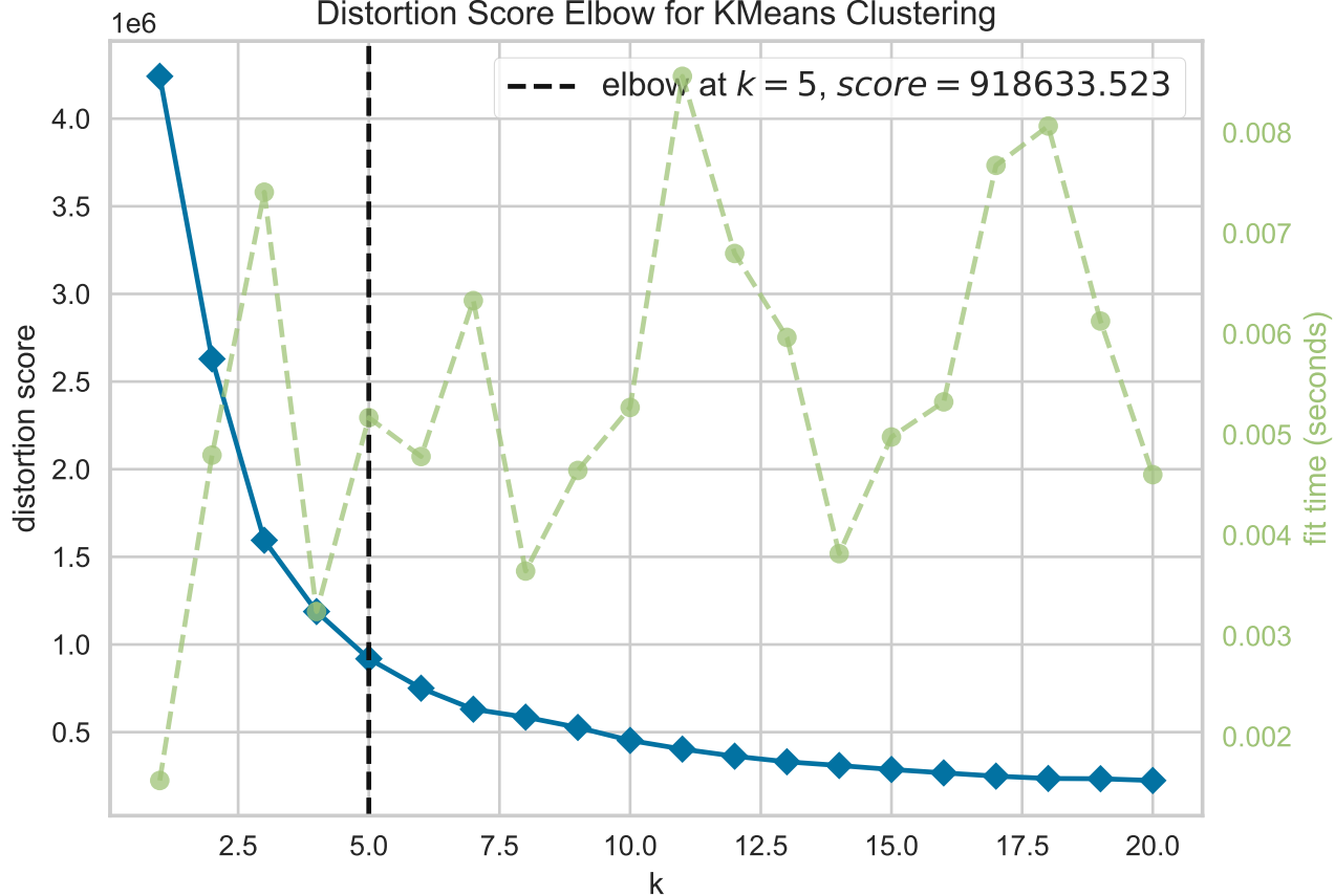
Distortion Score Elbow for KMeans Clustering
