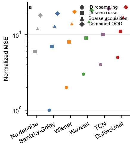
Distribution-shift performance
