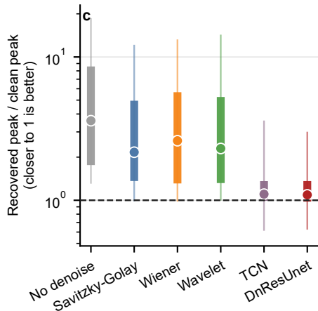
Weak-anomaly amplitude retention
