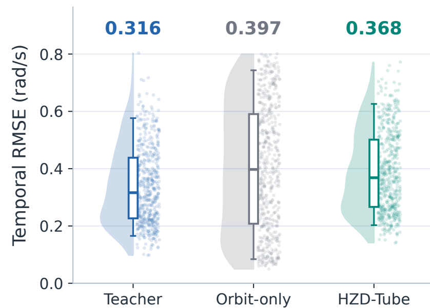
(f) \omega_z tracking error
