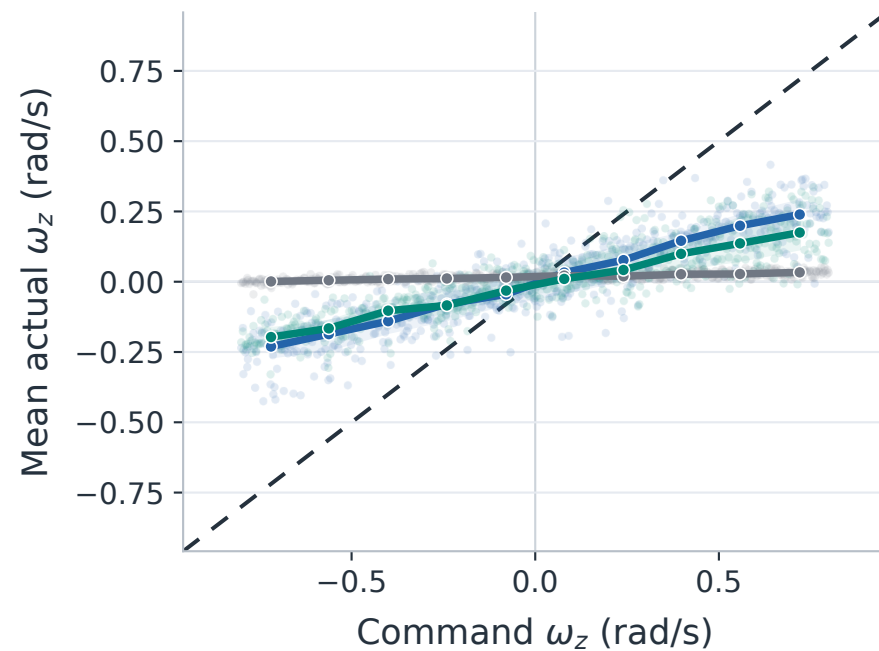
(f) \omega_z tracking error
