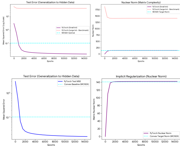
Figure 5. Implicit regularization effect of near-origin initialization in asymmetric BM matrix completion.
