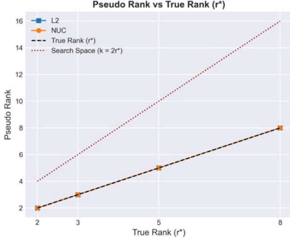
Figure 10. Both penalties recover rank exactly equal to r^* across all tested values, with the search-space ceiling k = 2r^* shown as reference.
