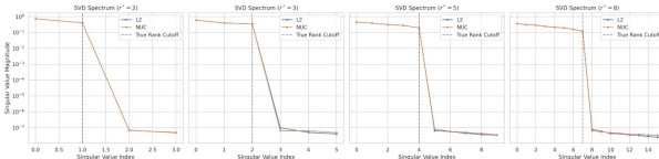
Figure 11. Singular values of W = UV^T at convergence, log scale. The cliff at index r^* separates kept singular values ( \mathcal{O}(0.1) to \mathcal{O}(1) ) from pruned ones ( \mathcal{O}(10^{-7}) ). L_2 and nuclear norm curves overlap.
