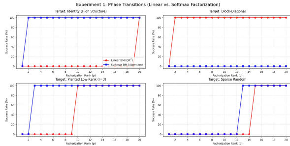
Figure 6. The Geometric Warp Drive: Softmax factorization induces massive structural compression.
