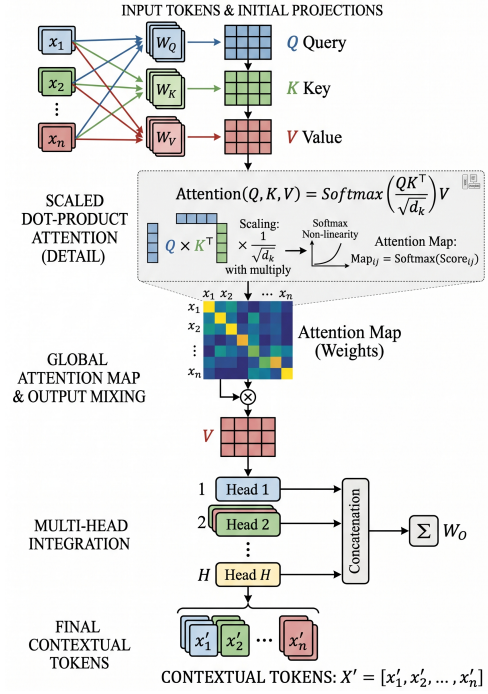
Figure 4. The Transformer architecture and self-attention mechanism.
