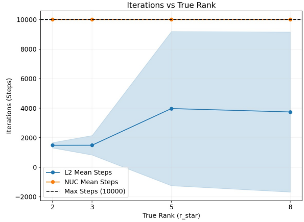
Figure 12. The L_2 runs converge under the early-stopping criterion well before the iteration budget is exhausted. The nuclear norm runs reach the maximum step count in every cell.
