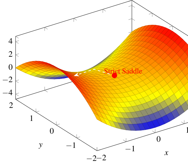
Figure 1. A strict saddle on the BM quotient manifold. The surface f(x, y) = x^2 - y^2 has zero gradient at the origin, yet a strictly negative Hessian eigenvalue in the y -direction creates a valley of descent. Stochastic noise projects onto this escape direction, guaranteeing that gradient descent exits the saddle.
