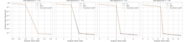
Figure 4. Singular values of W = UV^T at convergence, log scale. The cliff at index r^* separates kept singular values ( \mathcal{O}(0.1) to \mathcal{O}(1) ) from pruned ones ( \mathcal{O}(10^{-7}) ). L_2 and nuclear norm curves overlap.
