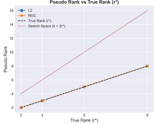
Figure 3. Both penalties recover rank exactly equal to r^* across all tested values, with the search-space ceiling k = 2r^* shown as reference.
