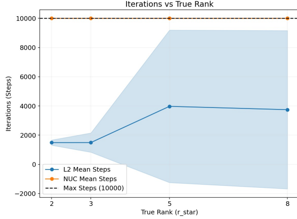
Figure 5. The L_2 runs converge under the early-stopping criterion well before the iteration budget is exhausted. The nuclear norm runs reach the maximum step count in every cell.
