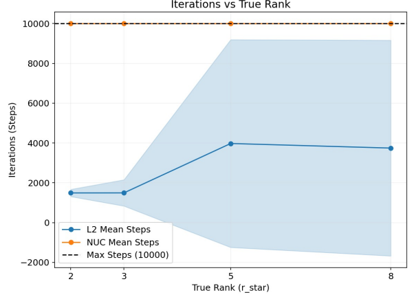
Figure 11. The L_2 runs converge under the early-stopping criterion well before the iteration budget is exhausted. The nuclear norm runs reach the maximum step count in every cell.
