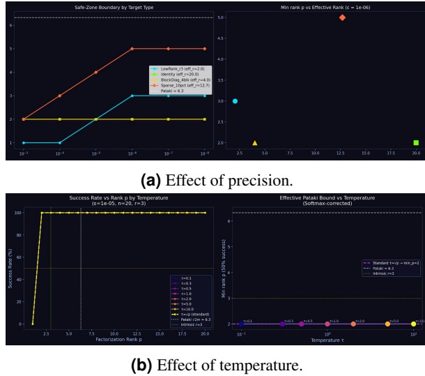
Figure 7. Empirical exploration comparing parameters on factorization success.
