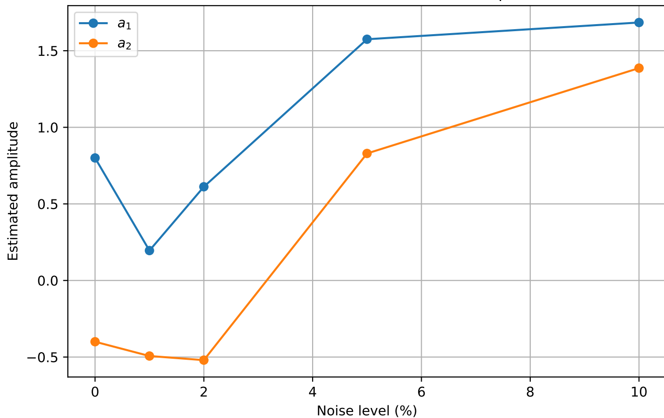
Effect of noise on estimated bedrock amplitudes
