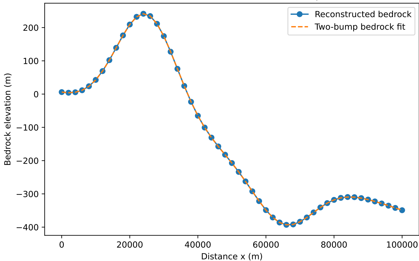
Bedrock reconstruction and two-bump fit
