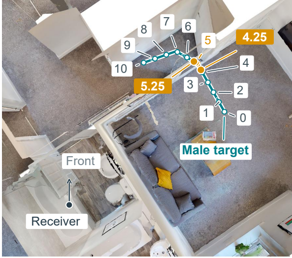
Single Moving Target
