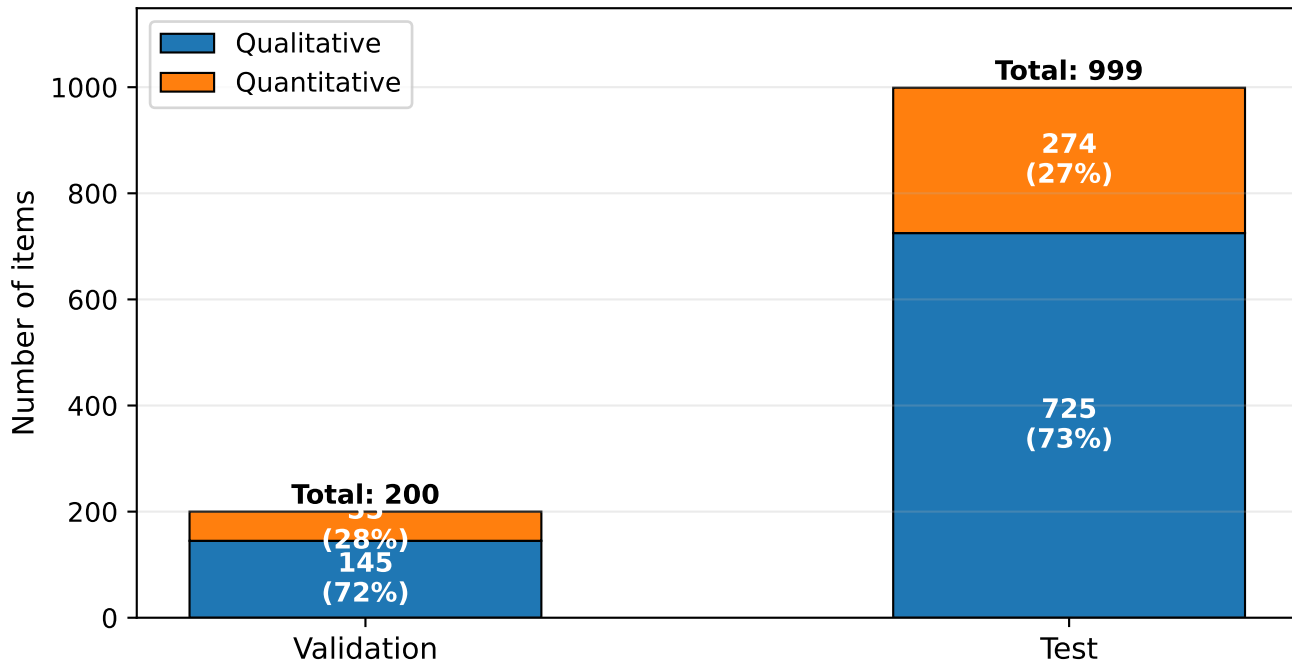
PhysBench-Diag composition (quant/qual partition)
