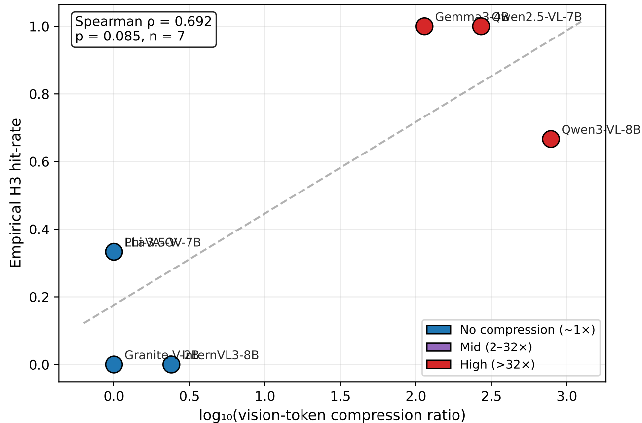
Architectural compression vs. empirical H3 hit-rate
