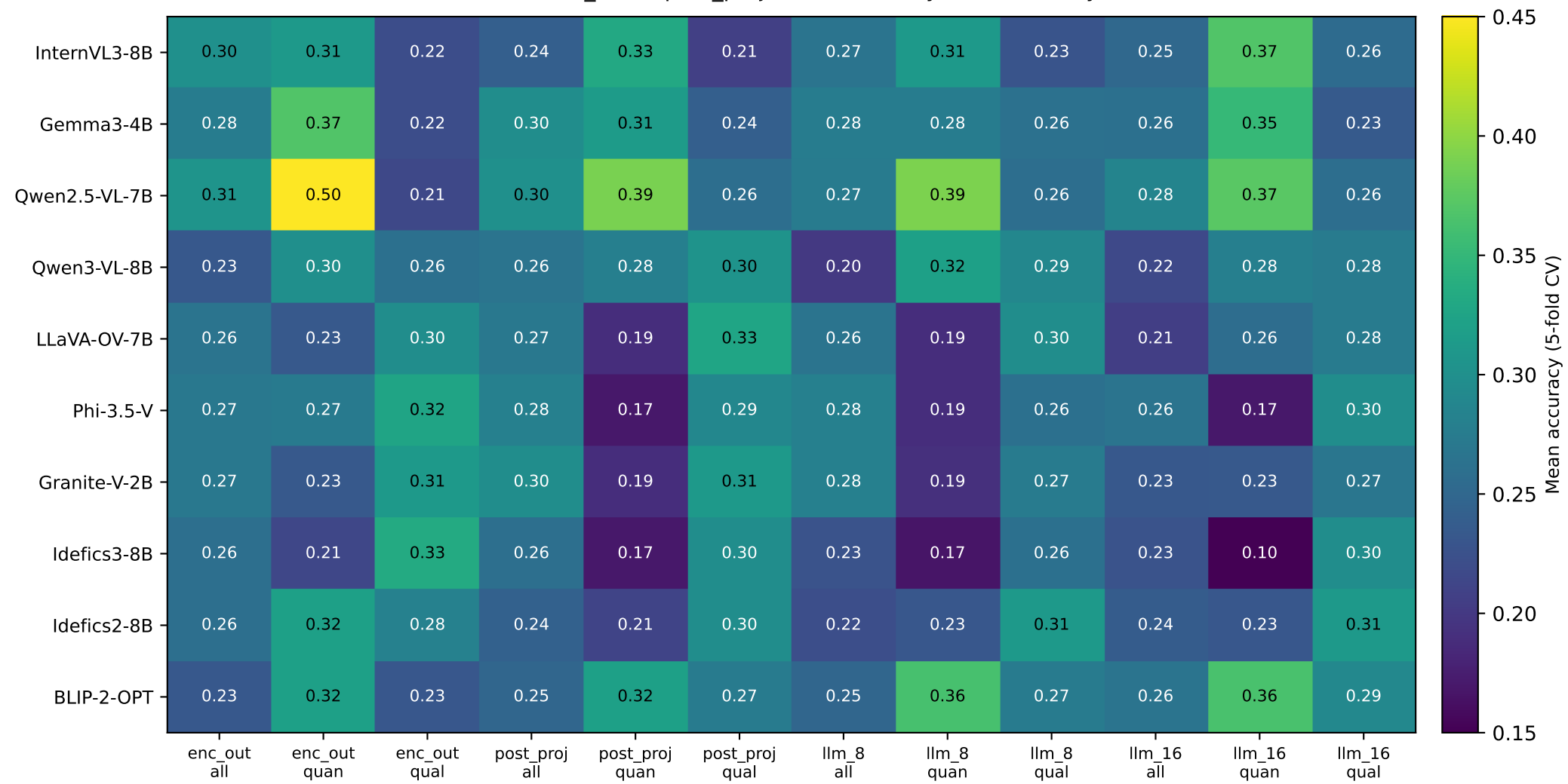
Probe accuracy on target='answer' (4-way A/B/C/D) Sites: encoder_out → post_projector → LLM layer 8 → LLM layer 16
