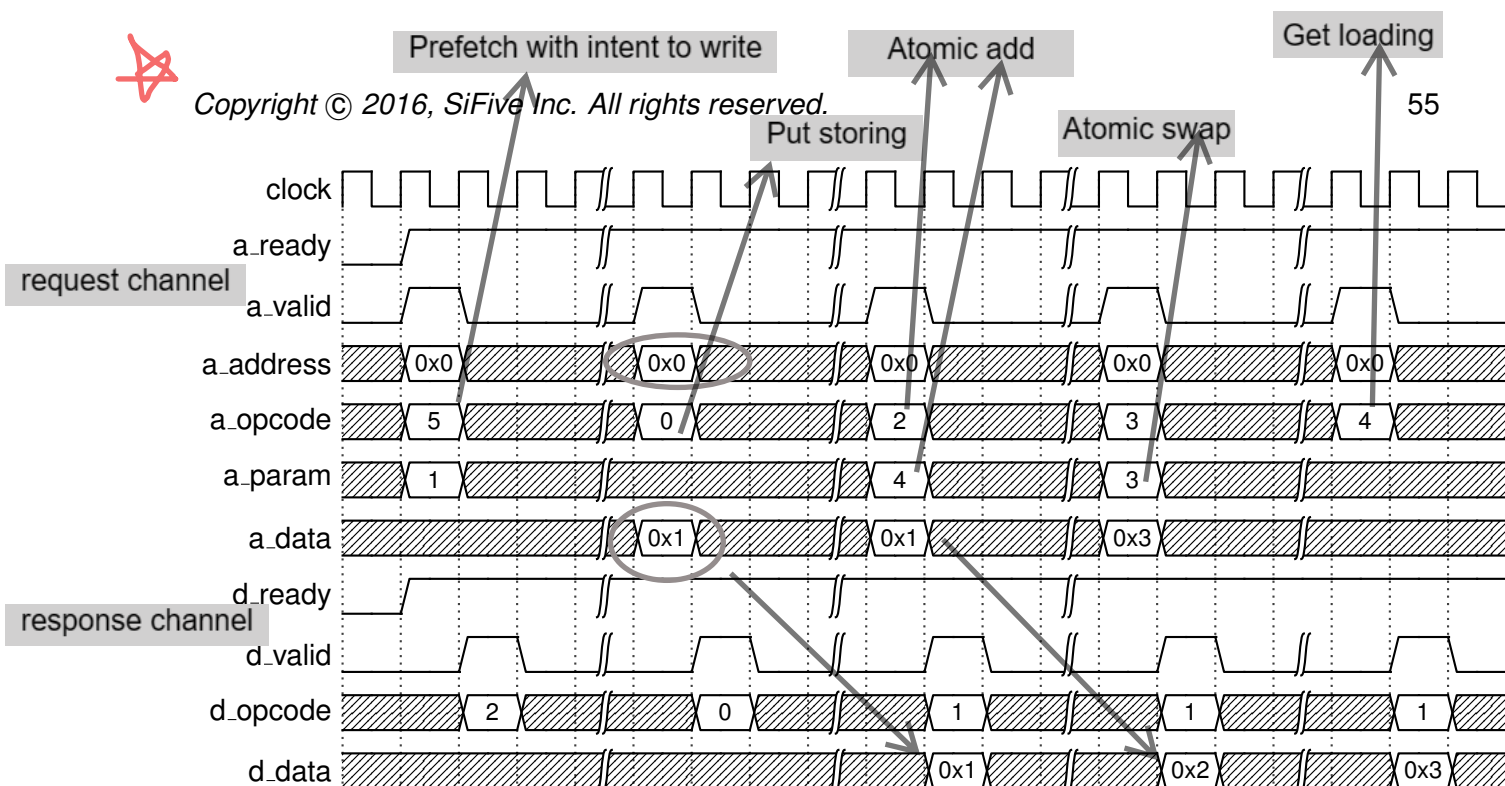
Figure 7.1: Waveform containing Atomic and Hint operations. Prefetch with intent to write; Put storing 0x1; Atomic add of 0x1 returning 0x1; Atomic swap of 0x3 returning 0x2; Get loading 0x3.
