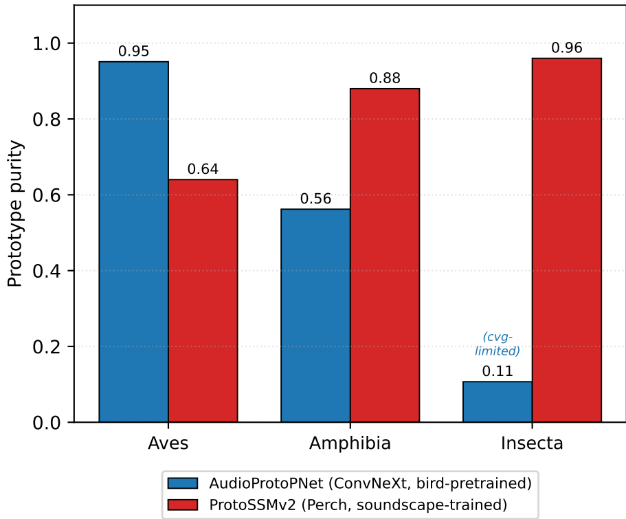
Inverted purity gradients by training domain
