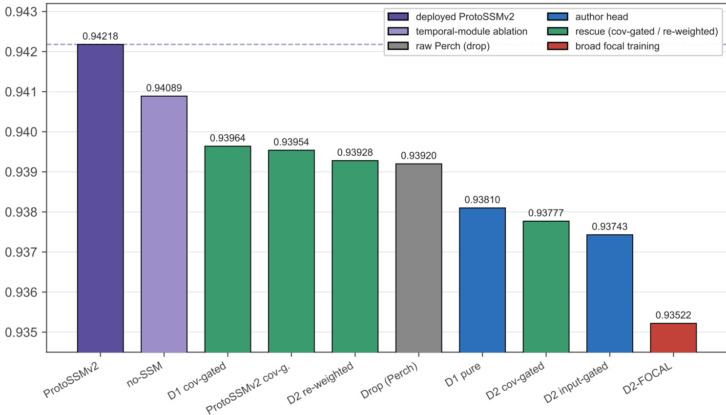
Private leaderboard (234-species macro-AUC)
