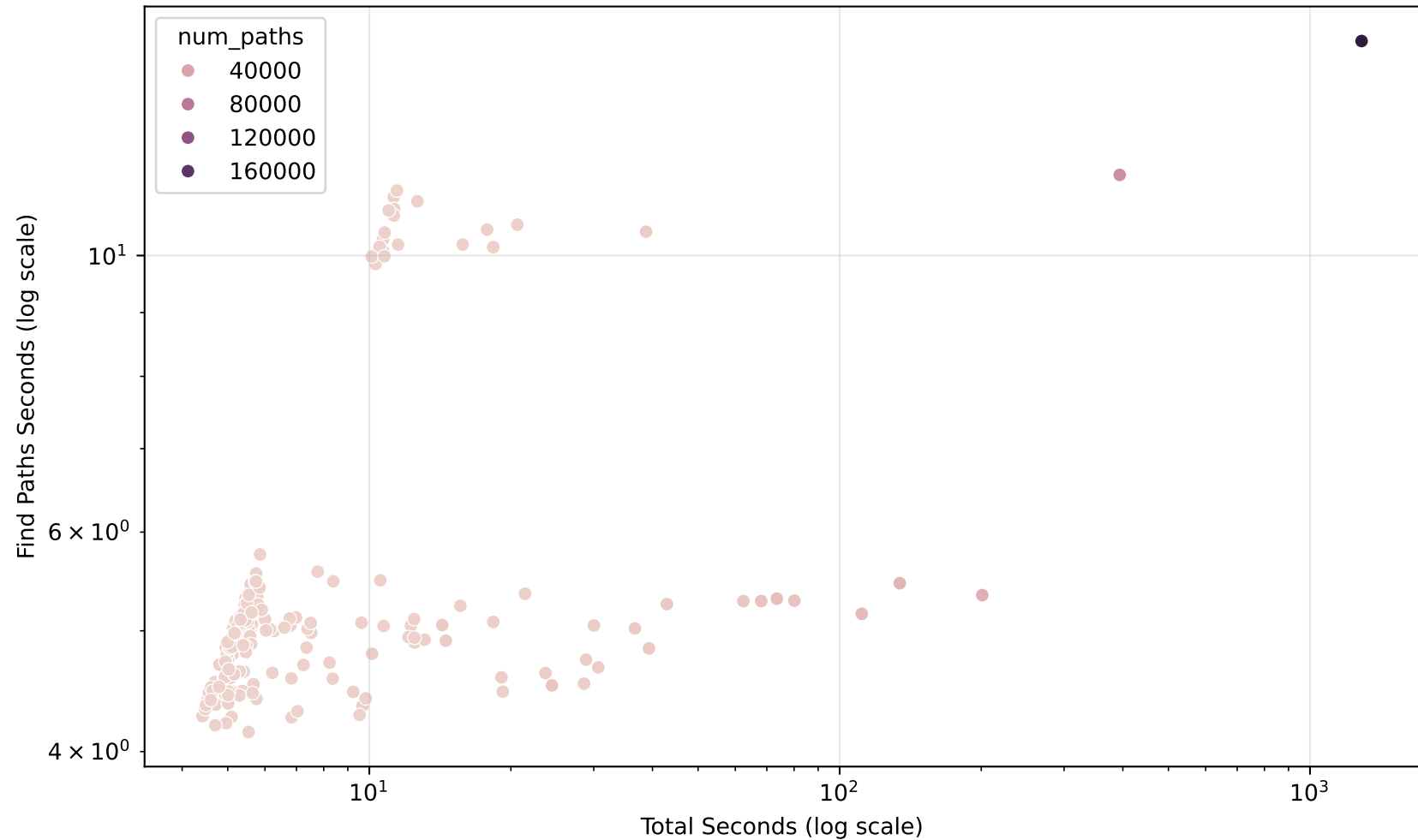
Total Time vs Path-Finding Time (Log-Log Scale)
