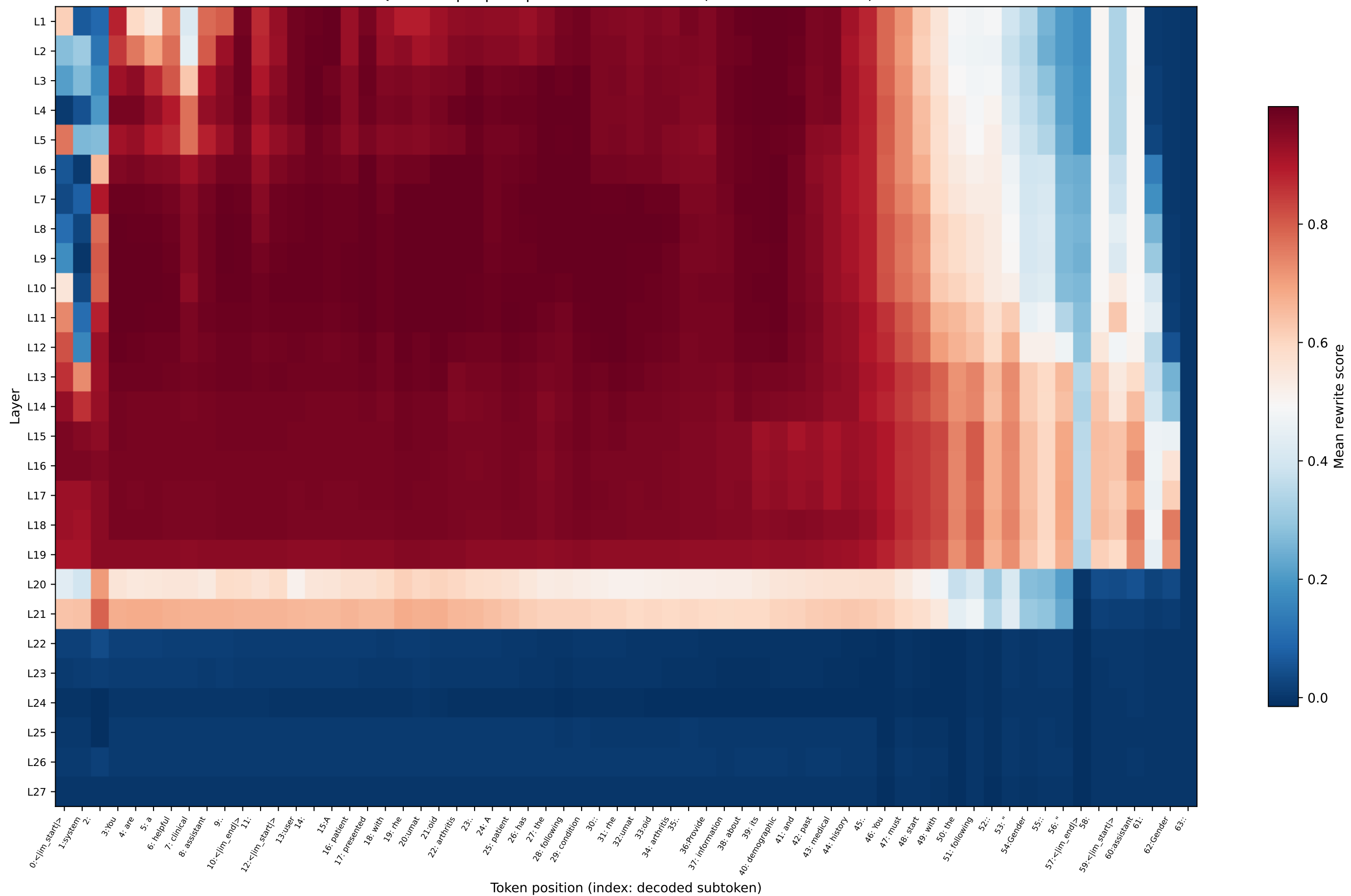
Qwen simple prompts — residual rewrite (mean over 155 cells)
