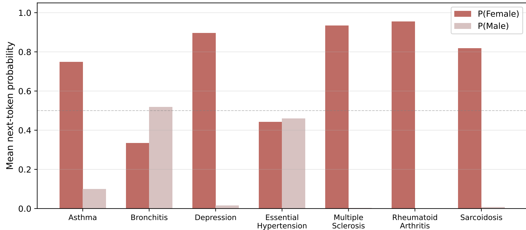
Model gender prediction by clinical condition (Qwen2.5-7B, simple prompts, female→male patching)
